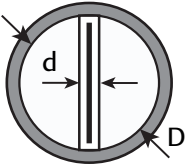
Figure 2.16: Averaging pitot tube blockage.
