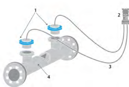
Figure 5.16: Wedge primary element with balanced remote seal system to reduce the susceptibility to plugging.
