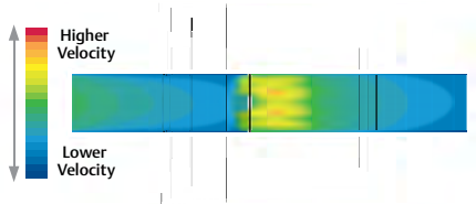
Figure 9.23: Energy conservation for a multi-hole orifice plate.
