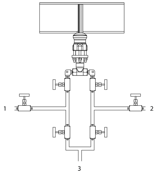
Figure 10.10: Arrangement of impulse piping for intermittent purge.
