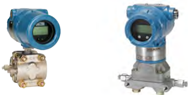
Figure 8.8: Biplanar (left) and Coplanar (right) process flanges for connecting a transmitter to the process.
