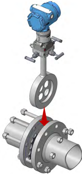
Figure 10.5: Wafer-mounted meter.
