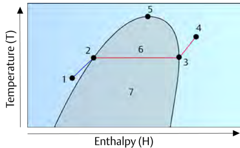
Figure 6.1: Mollier diagram showing the transition from water to steam as heat is added.
