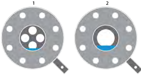
Figure 4.17: A Conditioning Orifice Plate has a much smaller dam height than a comparable traditional orifice plate.
