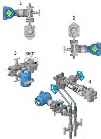
Figure 10.27: Orientation for the Rosemount 1195 with pipe and flanges removed for clarity.
