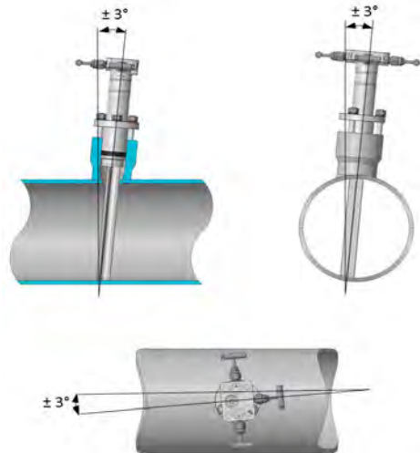
Figure 10.33: Annubar primary element alignment tolerances.
