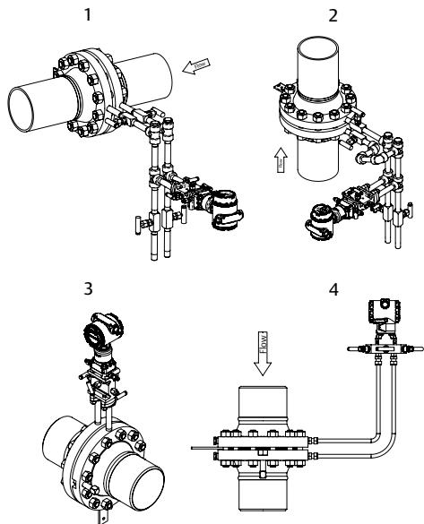
Figure 10.30: Orifice plate flow meters for remote mounting.
