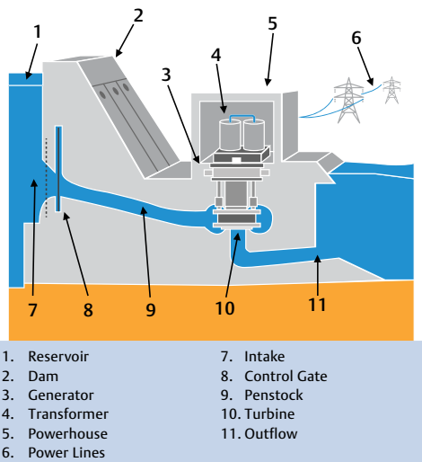
Figure 5.14: A typical hydroelectric power plant installation.
