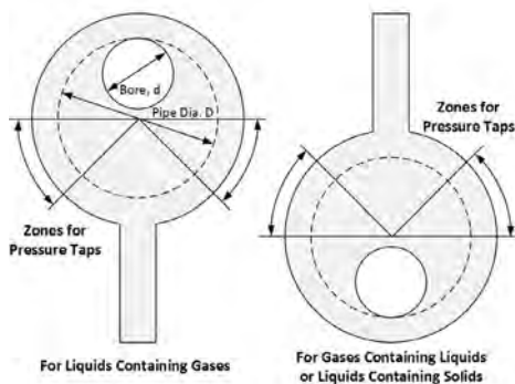
Figure 7.12: The eccentric orifice plate.
