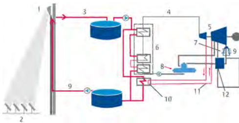
Figure 6.23: Diagram of routing and heat in a concentrated solar power facility.
