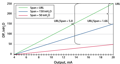
Figure 8.15: A changing DP transmitter span with a URL of 250 inH 2 O (62.2 kPa) and a span of 150 and 50 inH 2 O (37.3 and 12.4 kPa).
