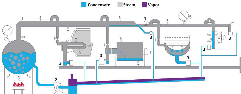
Figure 6.3: A typical saturated steam system.
