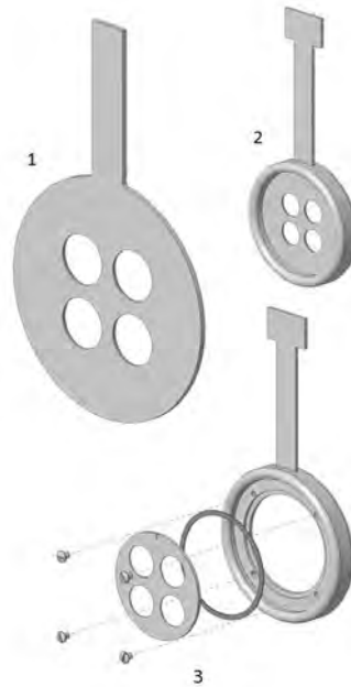
Figure 9.28: Rosemount 1595 Conditioning Orifice Plate models for paddle and universal for ring-joint flanges.
