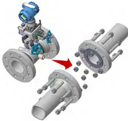
Figure 10.4: Spool-mounted meter.
