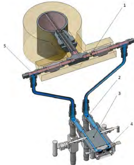
Figure 6.12: Cross section of an averaging pitot tube for steam applications in a vertical pipe.
