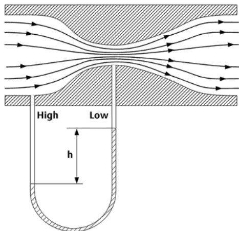
Figure 1.4: A DP flow meter using a U-tube manometer to measure the differential pressure.
